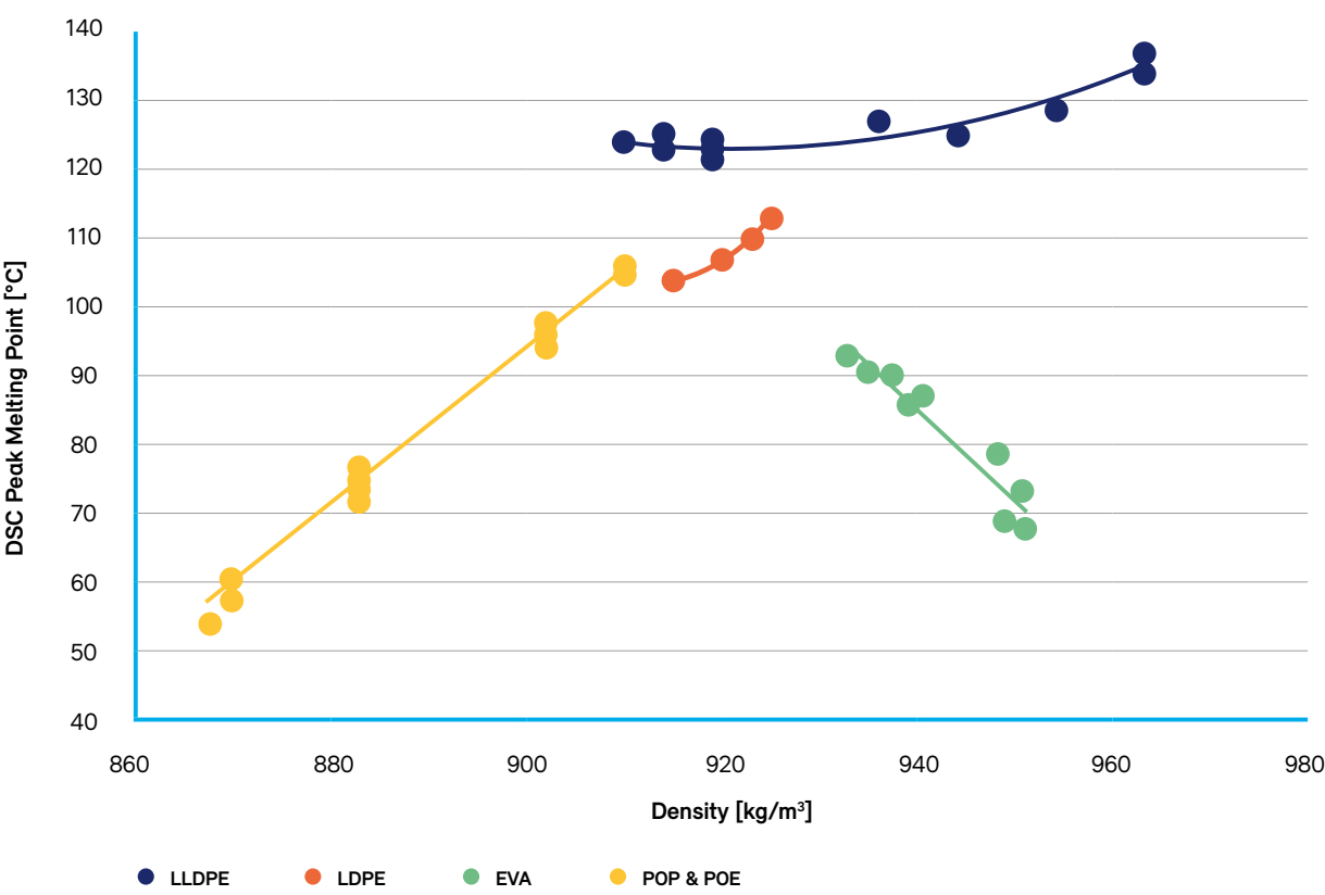
DSC Peak Melting point Plastomers, Elastomers, LLDPE, LDPE and EVA
