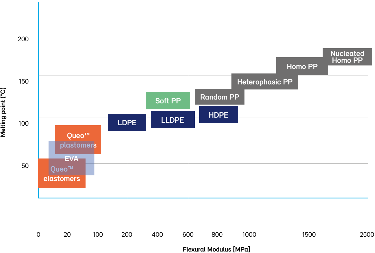
Melting Point vs. Stiffness (Flexural Modulus) for a wide array of PO materials
