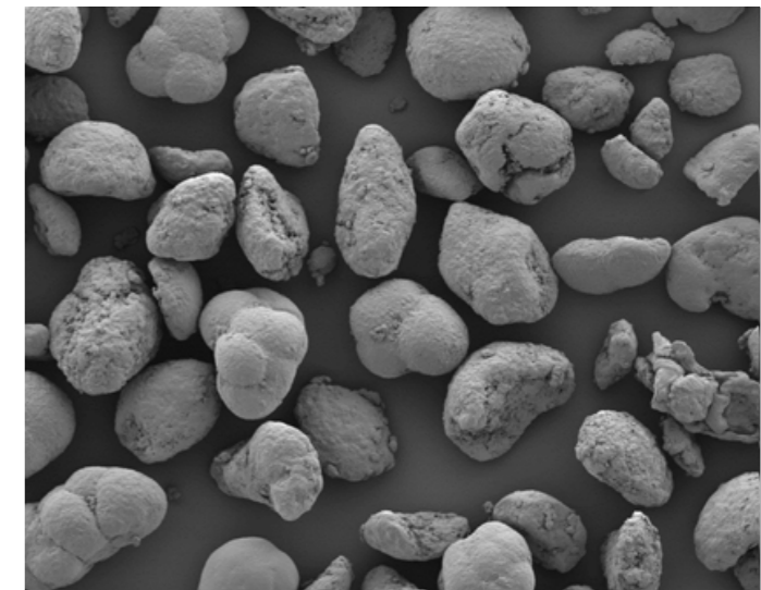
Figure 7: SEM microscopy image of Borealis HC001A-B1 grade, available in powder form.
