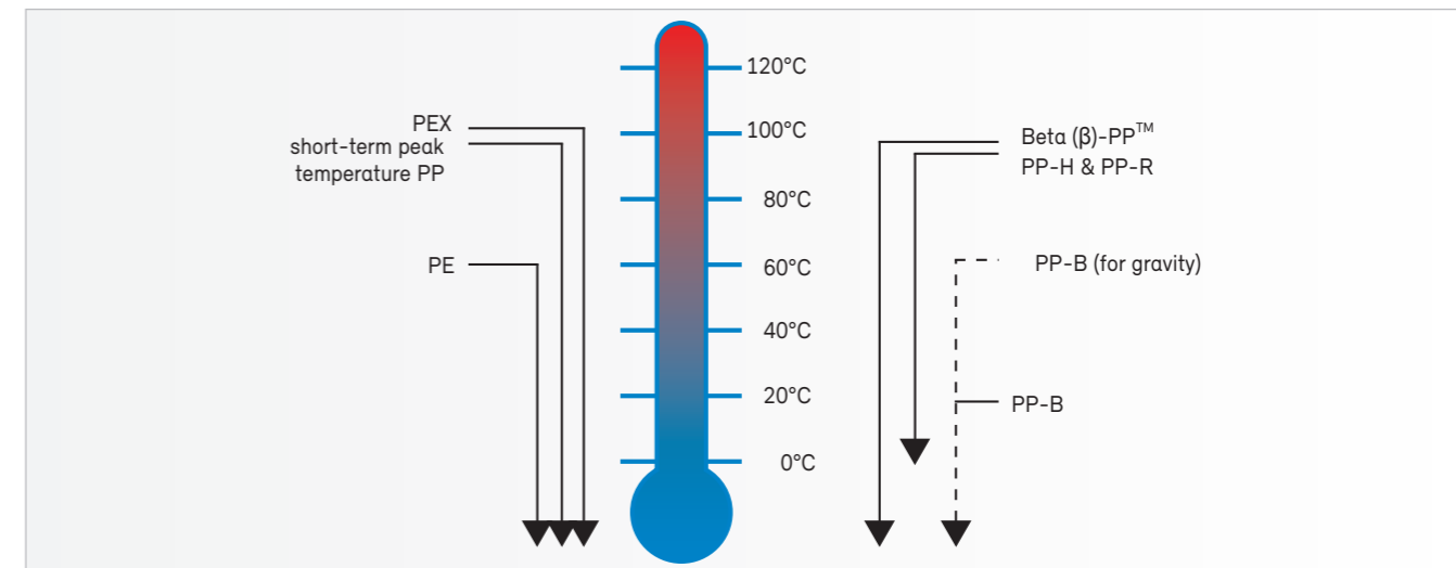
BE60-7032 has an increased operating temperature
