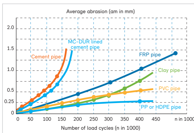
Darmstadt test method to determine surface abrasion
